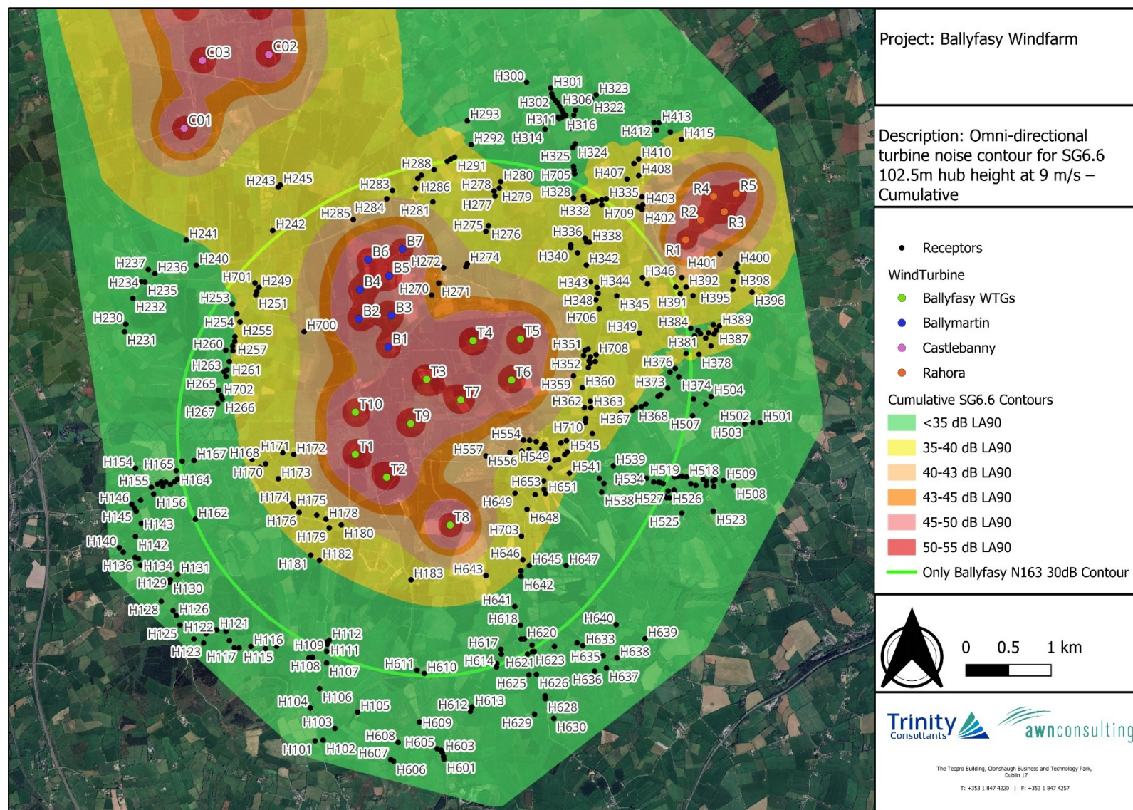
Figure A12-2 Omni Directional noise prediction contour SG6.6 102.5m – Cumulative Contours
