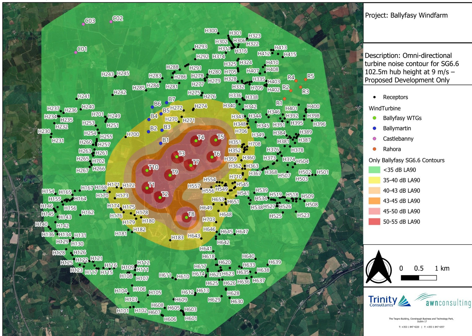
Figure A12-1 Omni Directional noise prediction contour SG6.6 102.5m – Proposed Development Only
