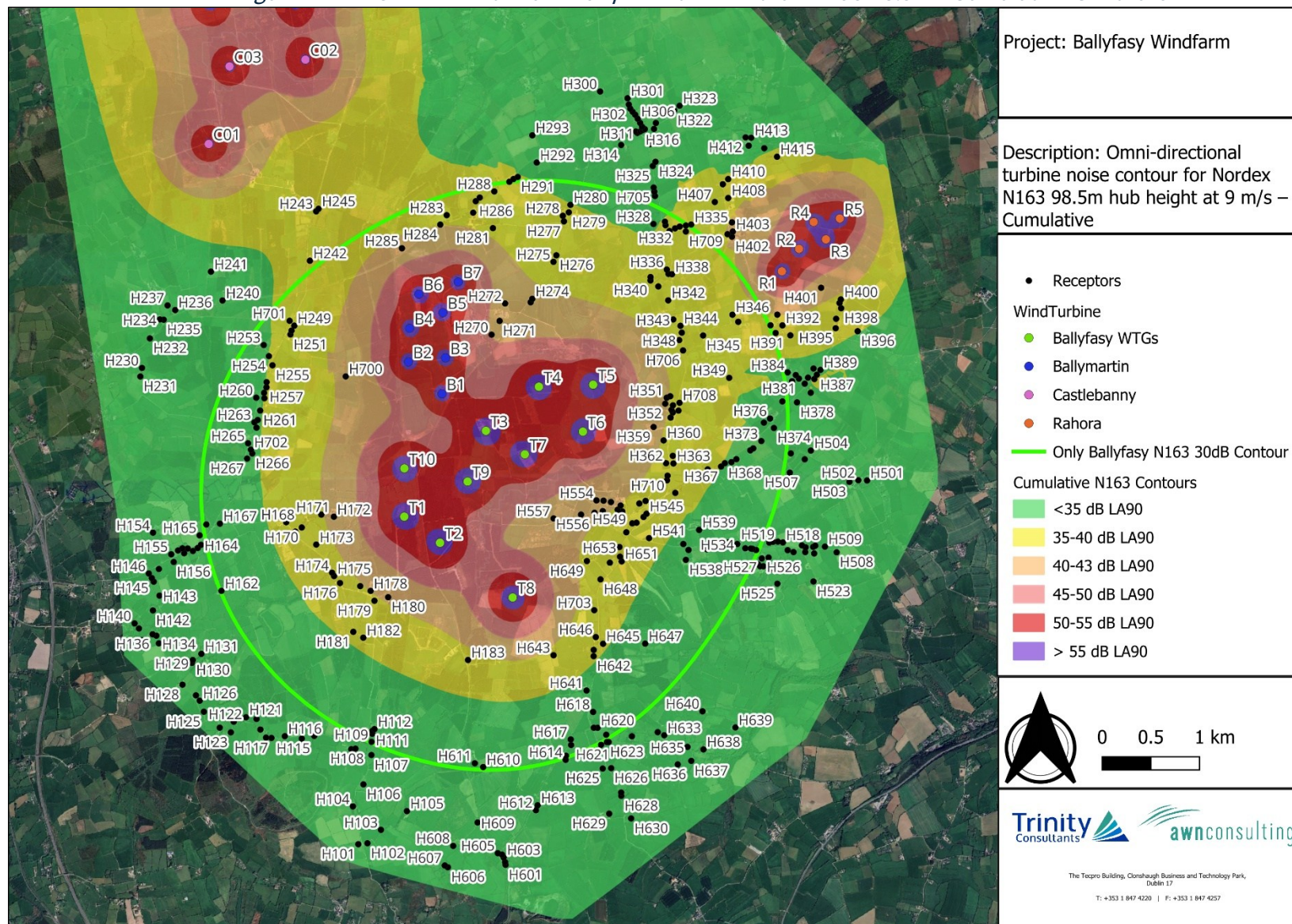
Figure A12-2 Omni Directional noise prediction contour N163 98.5m– Cumulative Contours
